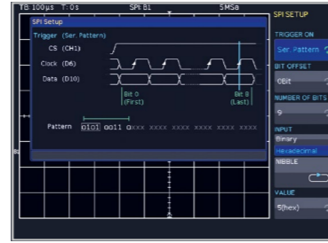
SPI bus trigger setup
