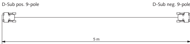
Fig. 11: RS-232C interface cable Type 1200A27
