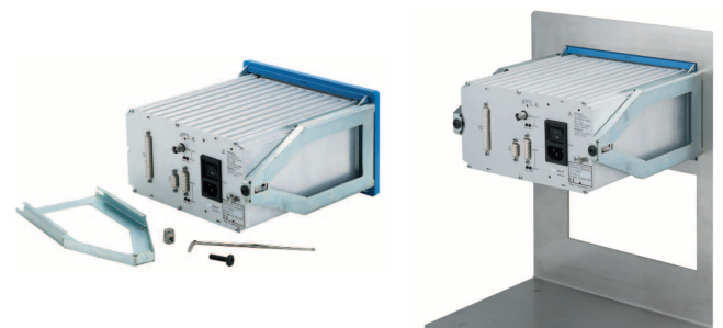
Fig. 10: Multi-channel charge amplifier in 19" cassette with panel mounting set Type 5070A2xxxx
